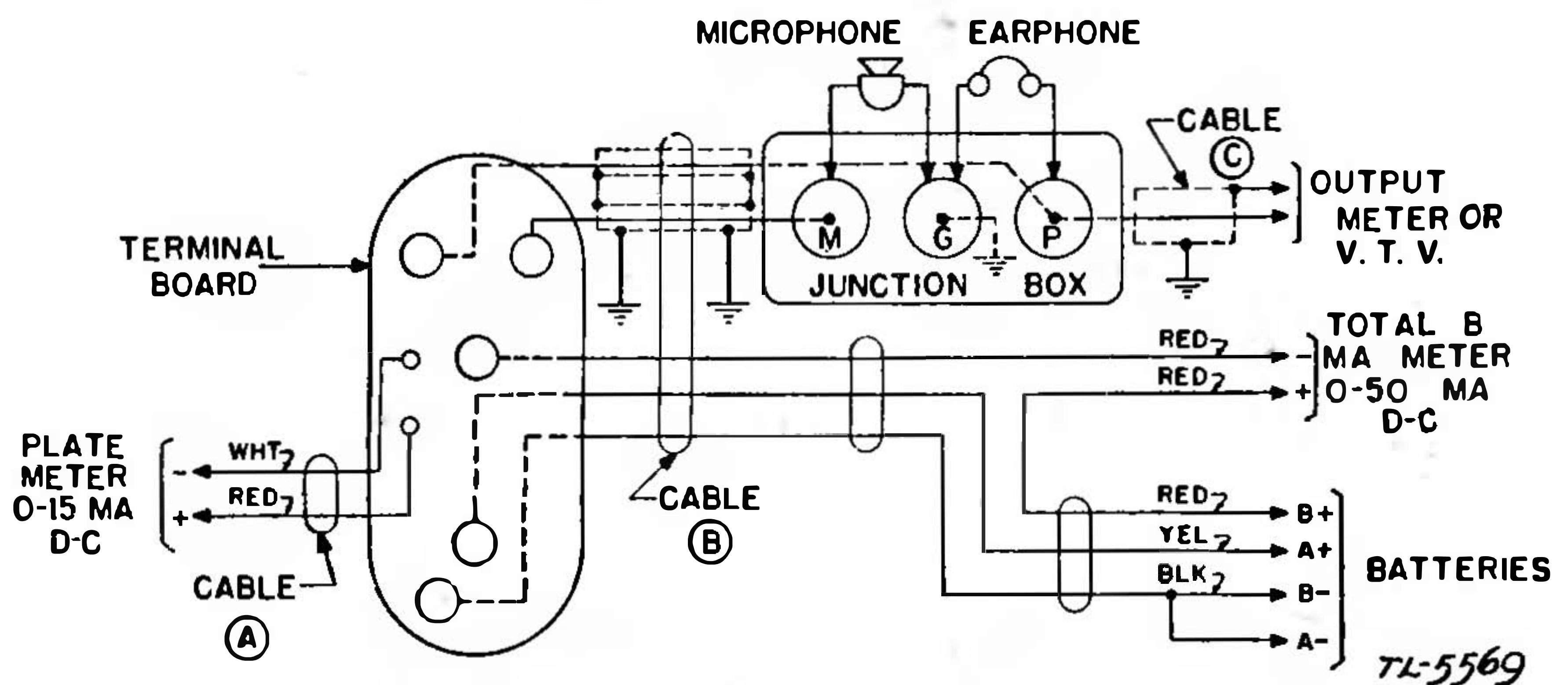
FIGURE 15.—Test equipment IE-15-A—harness connections.
